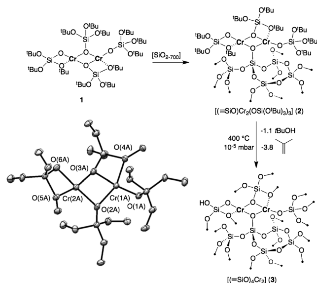
Scheme 2. Grafting of 1 on SiO 2-700 to form [(≡SiO)Cr 2 (OSi( tert Bu) 3 ) 3 ] ( 2 ) and thermal decomposition under high vacuum to yield [(≡SiO) 4 Cr 2 ] ( 3 ). The solid-state structure obtained by X-ray diffraction for an independent molecule of 1 is shown at 50% probability. Methyl groups of –OSi( tert Bu) 3 ligands and H atoms have been removed for clarity.
