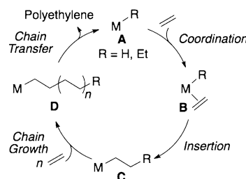
Scheme 1. Generally accepted mechanism for ethylene polymerization by metal–alkyl complexes.
